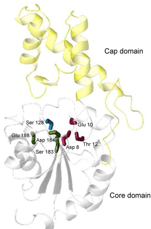
Figure 3. Model of E1 enolase/phosphatase based on sequence homology with \beta -phosphoglucomutase (PDB entry 1LVH). 22 Modeling was accomplished using the nest subroutine of the program Jackal. 28 The positions of proposed active site residues are shown and labeled. These correspond to the strongly conserved residues shown in Figure 4, and are color-coded to correspond to Figure 4. Figure was generated using MOLMOL. 29
